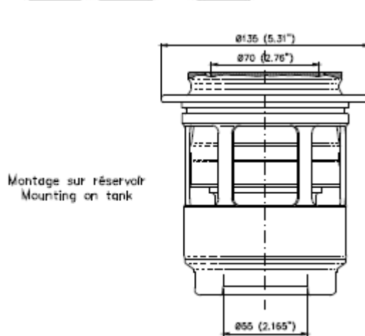
Female Coupling
